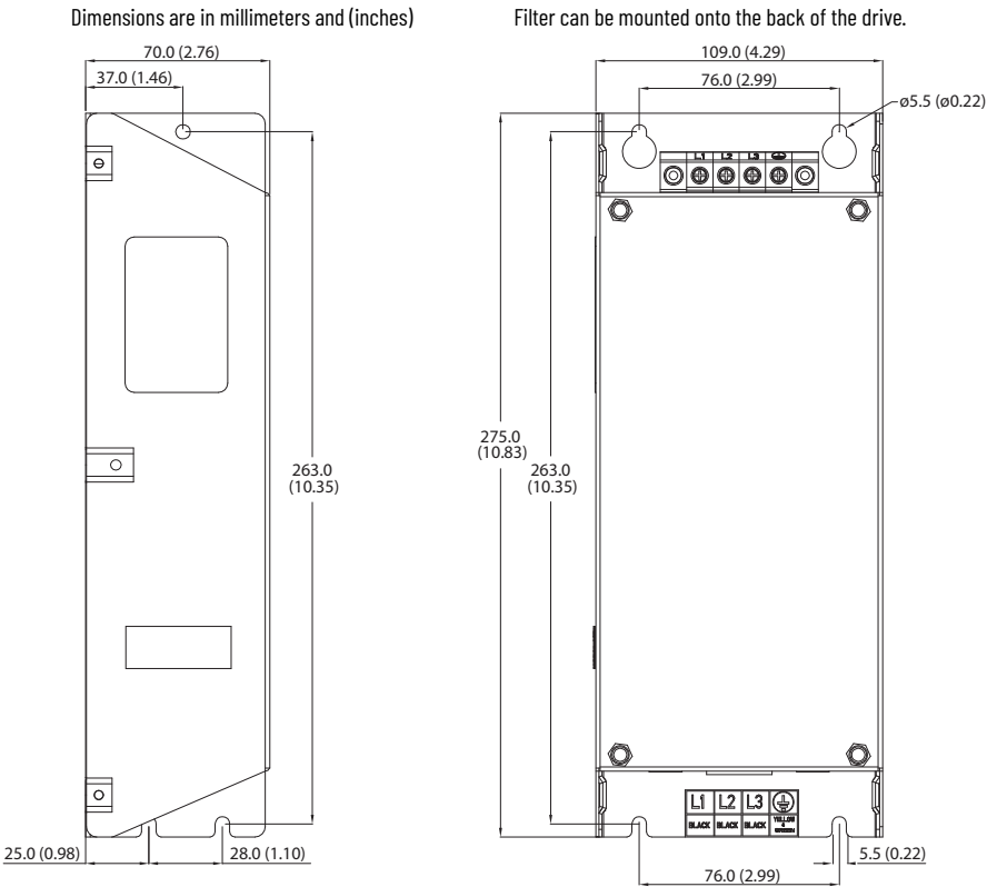
Figure 45 - EMC Line Filter Dimensions – Frame D
