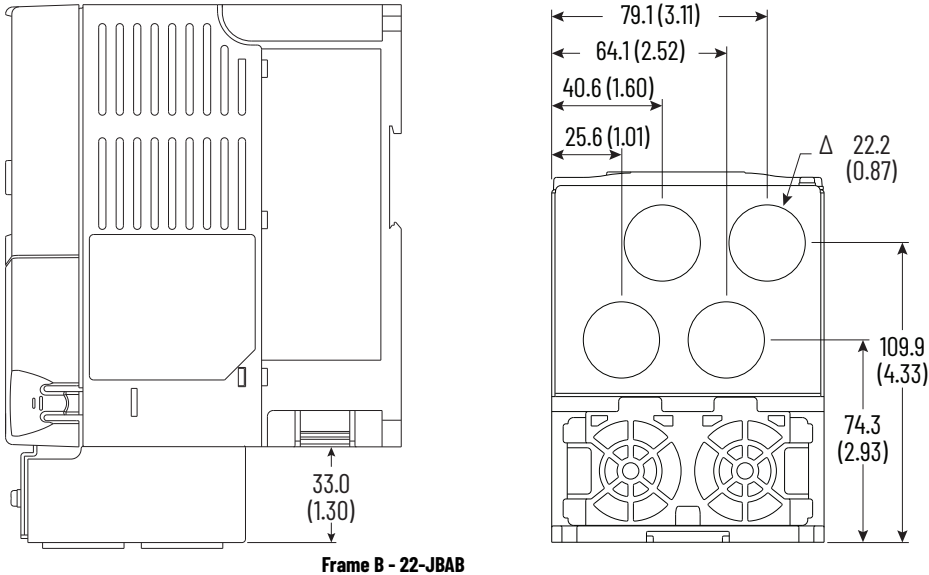
Figure 8 - IP30, NEMA/UL Type 1 Option Kit without Communication Option
