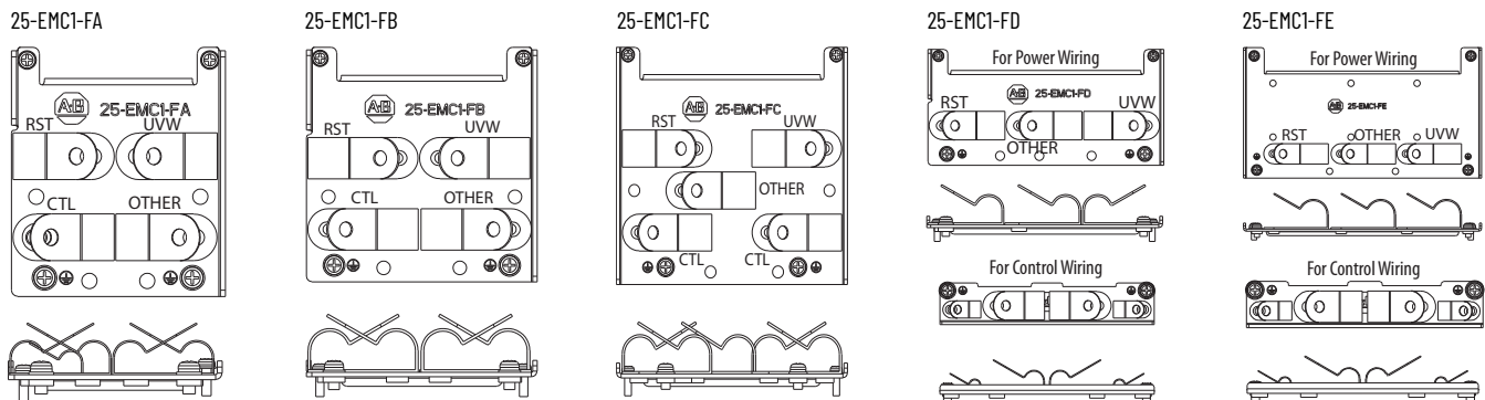
Figure 47 - PowerFlex 525 EMC Plate Dimensions
