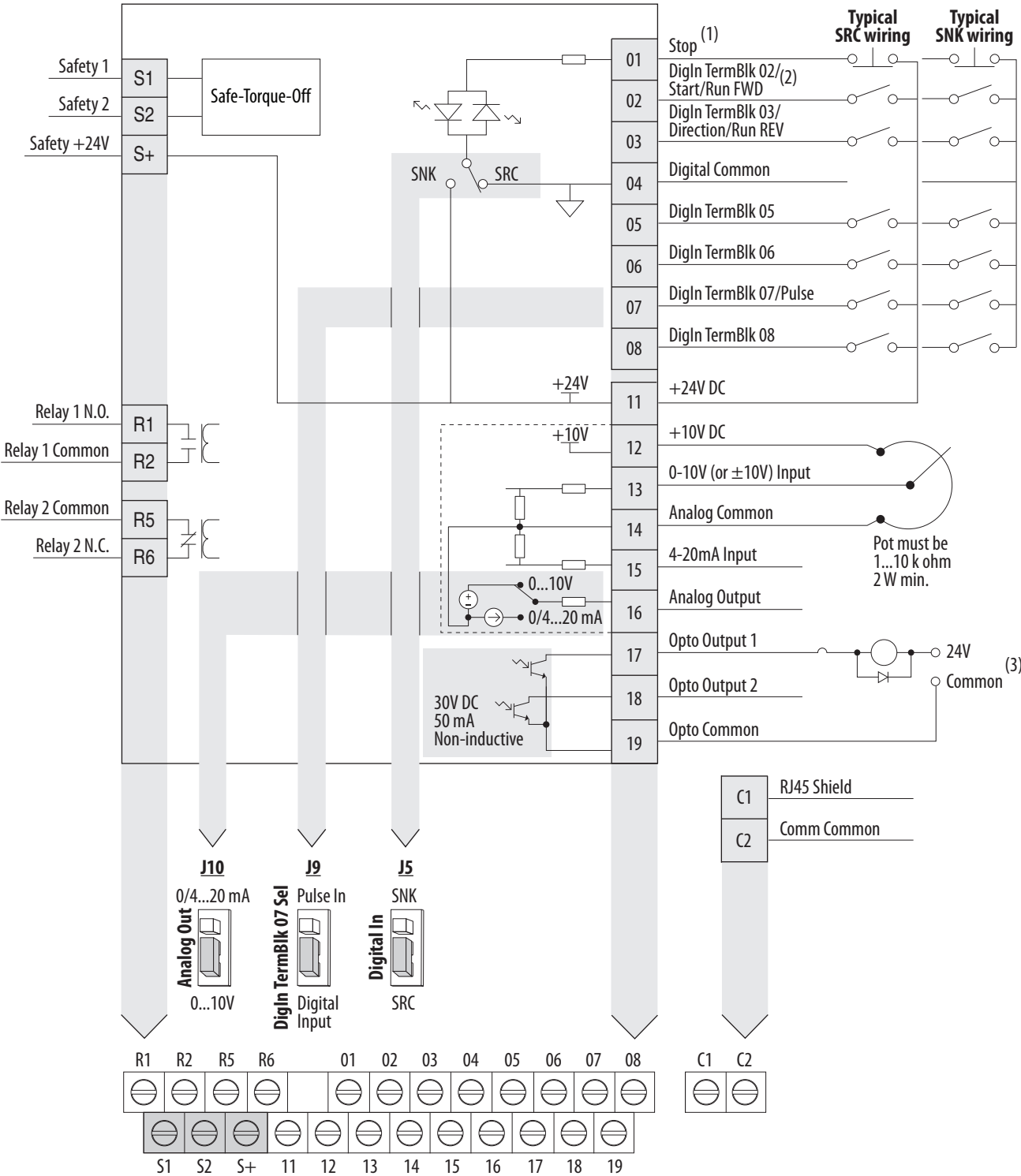
Figure 27 - PowerFlex 525 Control I/O Wiring Block Diagram
