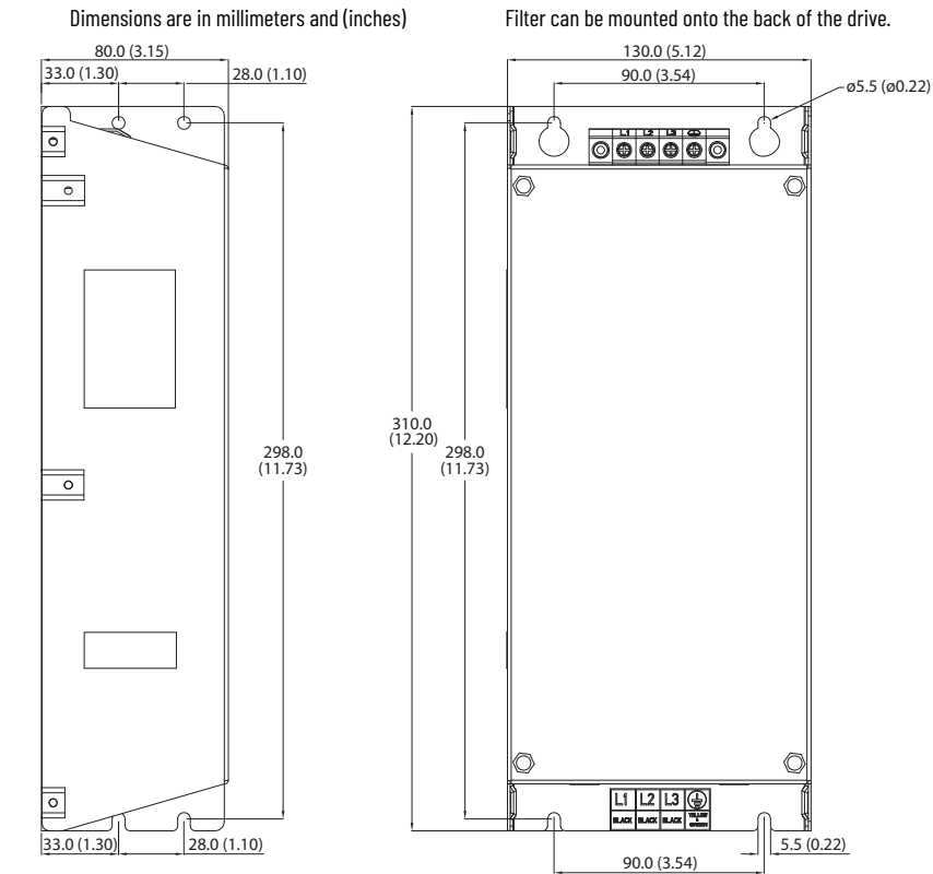
Figure 45 - EMC Line Filter Dimensions – Frame D
