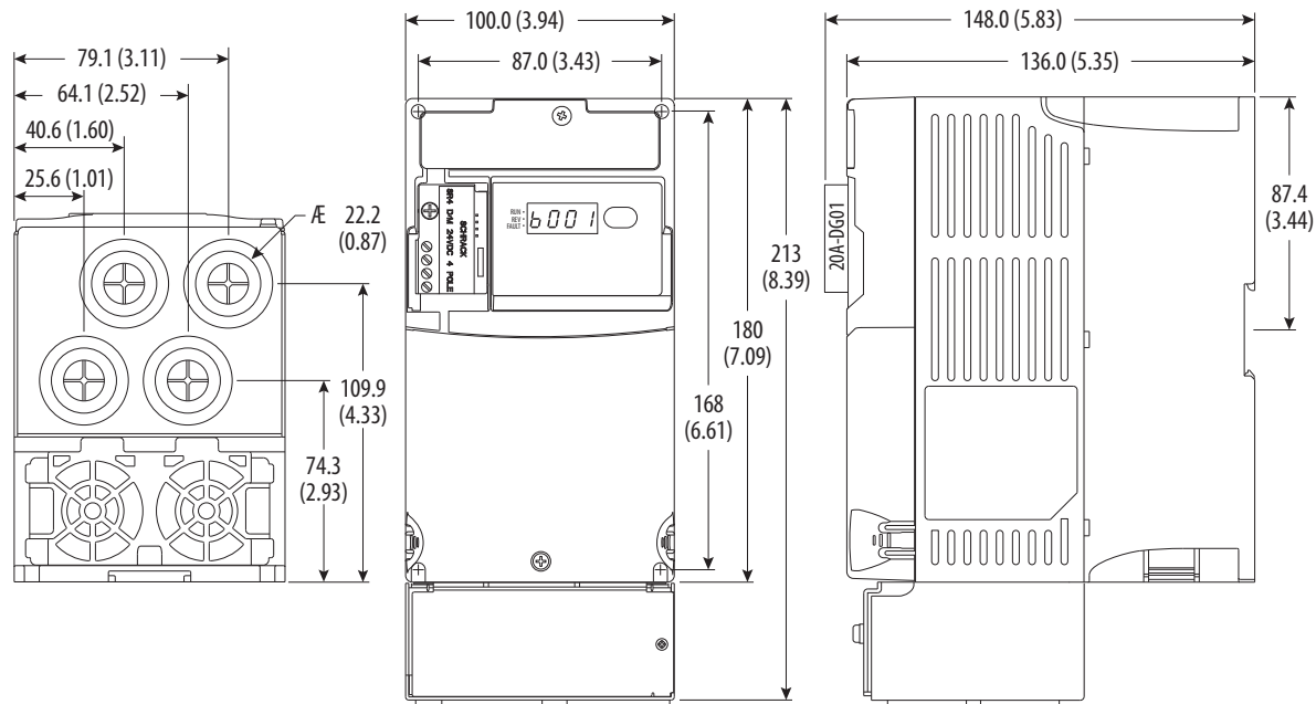
Frame B - 22-JBAB
