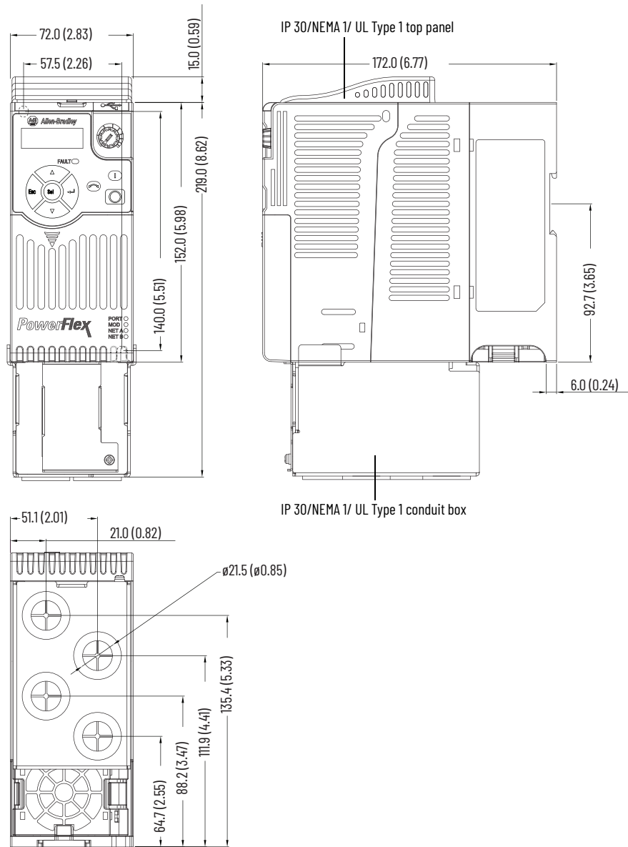
Figure 19 - IP 30/NEMA 1/UL Type 1 - Frame A
