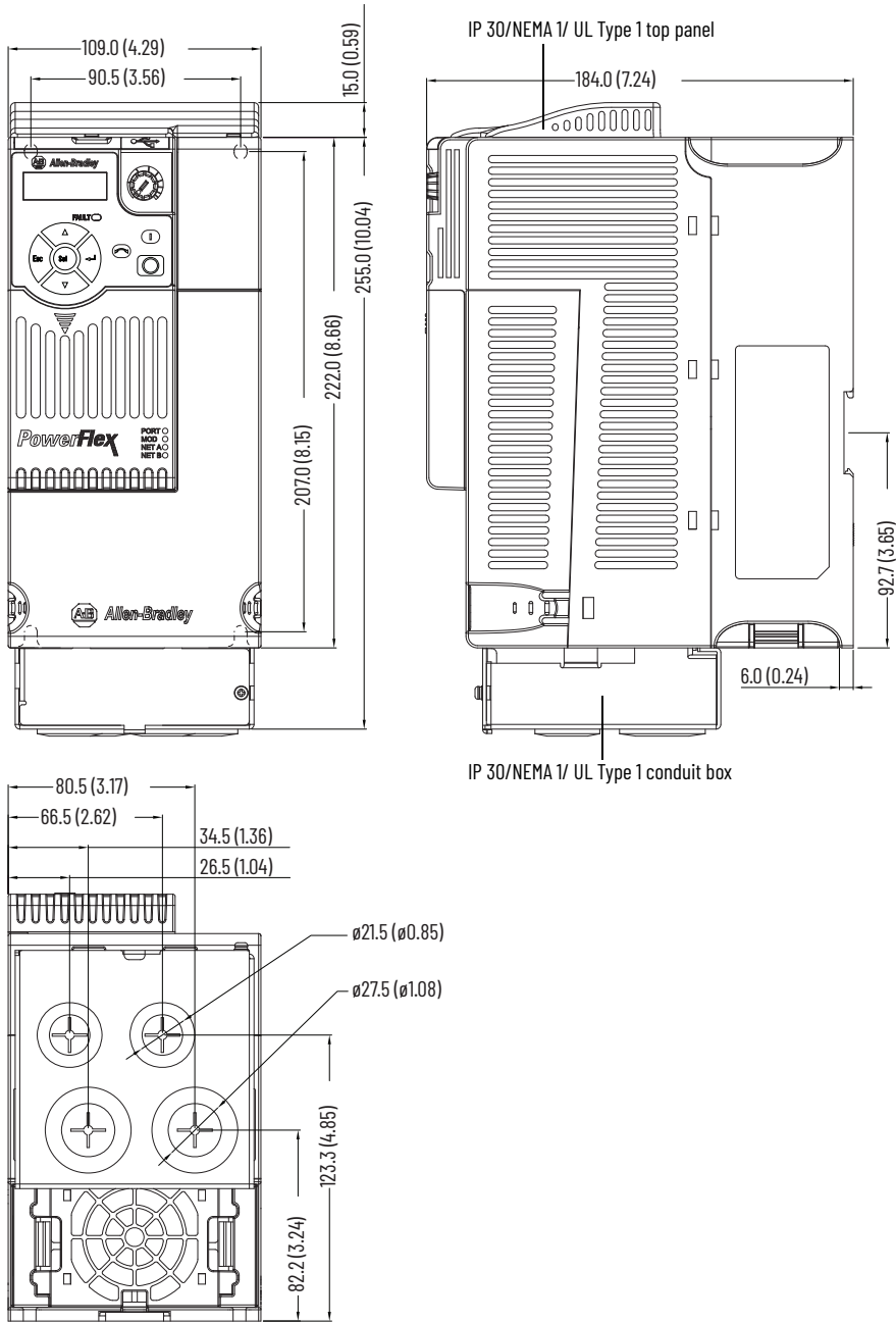
Figure 21 - IP 30/NEMA 1/UL Type 1 - Frame C
