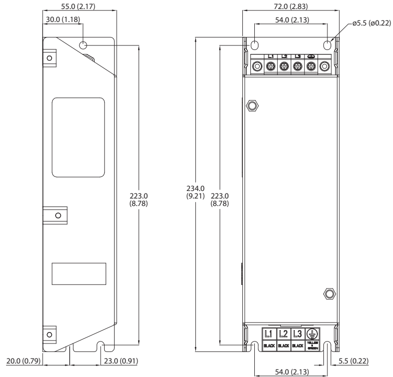
Figure 43 - EMC Line Filter Dimensions - Frame B
