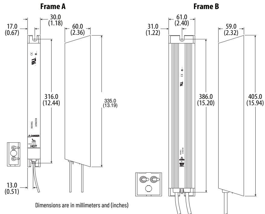
Figure 35 - Dynamic Brake Modules
