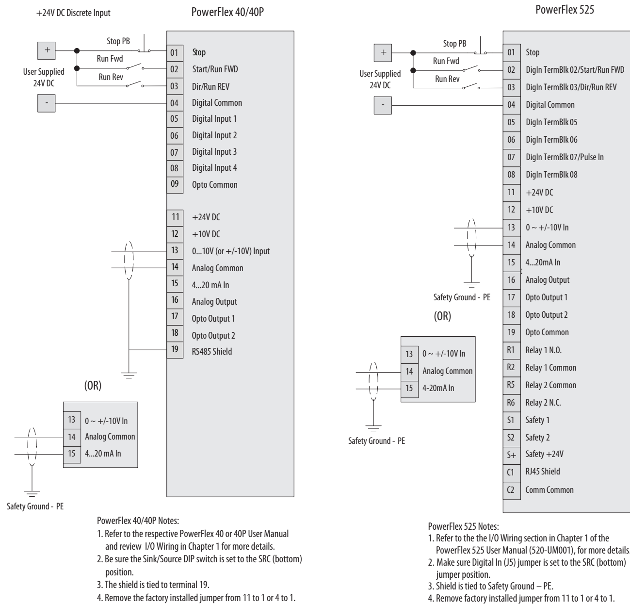
Figure 52 – 2 Wire Control (SRC), Analog Input Reference Wiring Example
