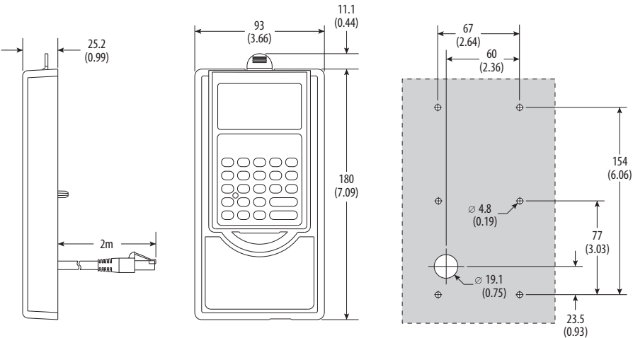
Figure 40 - NEMA Type 1 Bezel
