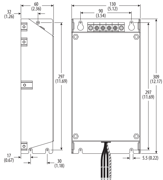
Figure 32 - Frame C EMC Line Filters
