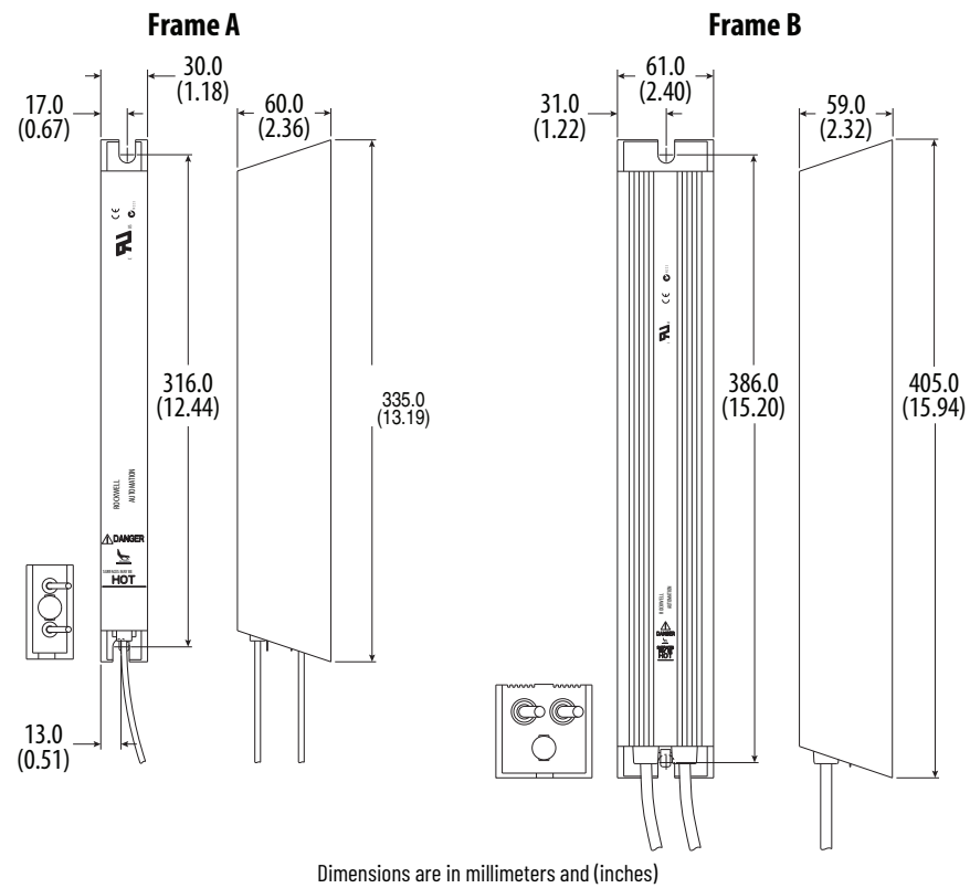
Figure 28 - Dynamic Brake Modules
