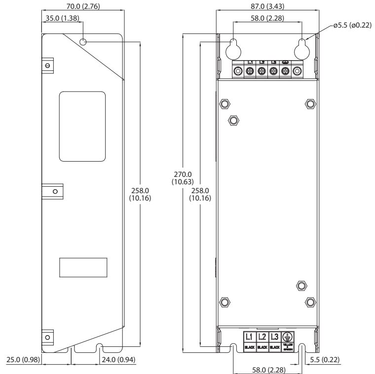
Figure 43 - EMC Line Filter Dimensions - Frame B
