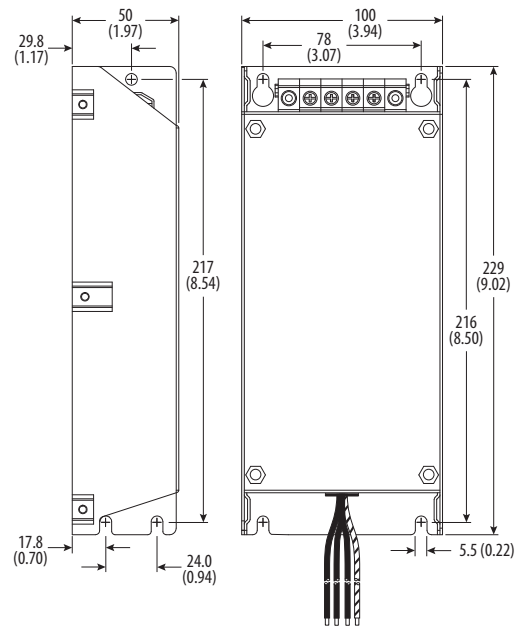
Figure 38 - Frame C EMC Line Filters
