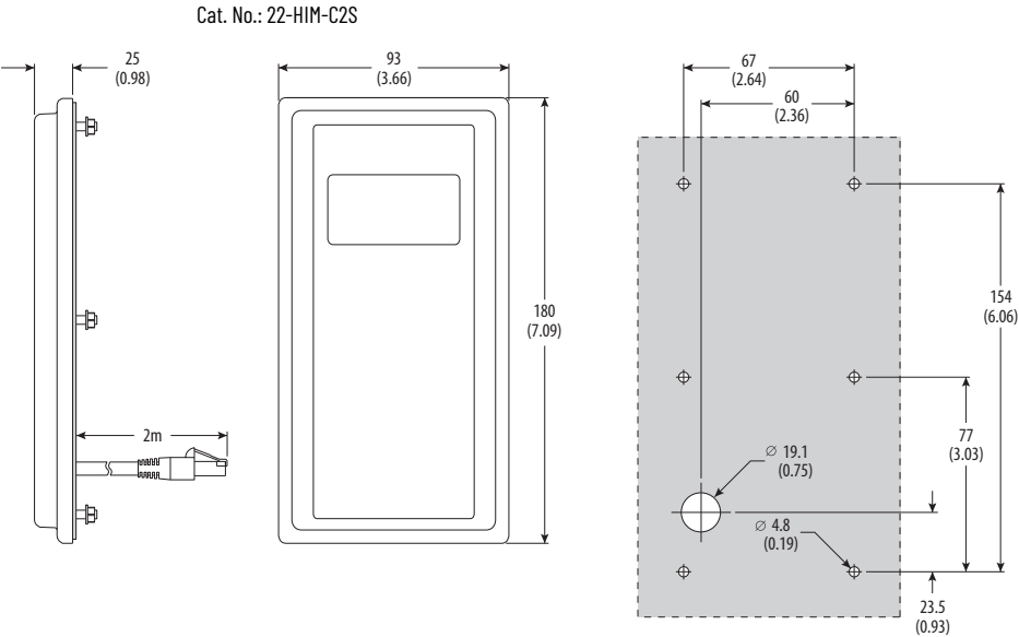
Figure 33 - Remote (Panel Mount) HIM
