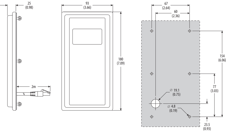
Figure 40 - NEMA Type 1 Bezel
