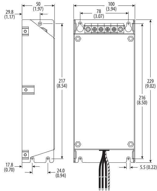
Figure 32 - Frame C EMC Line Filters
