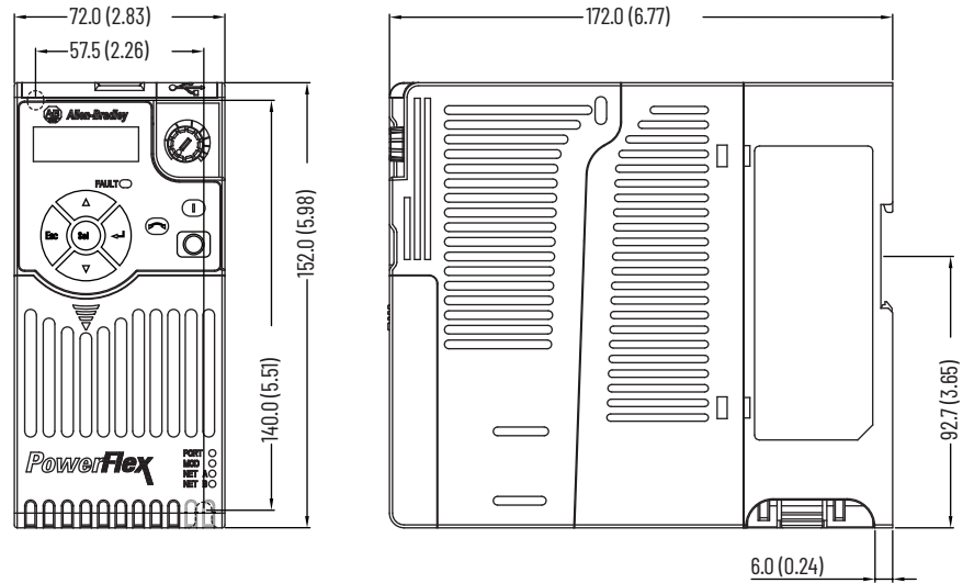
Figure 13 - IP 20/Open Type - Frame B
